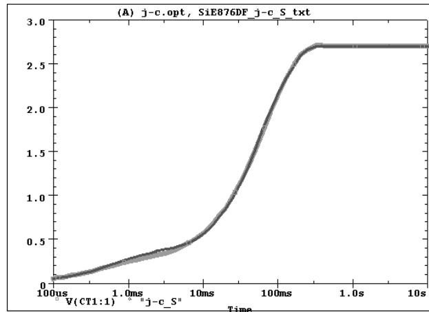
SiE876DF Tank j-c Source Temperature:27.0
