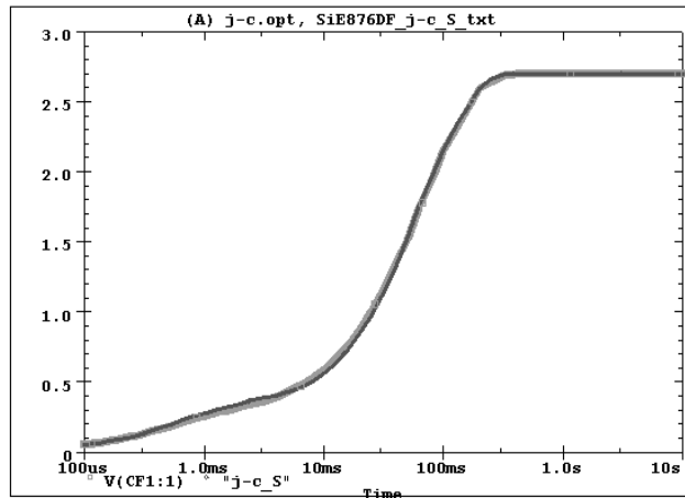
SiE876DF Filter j-c Source Temperature:27.0
